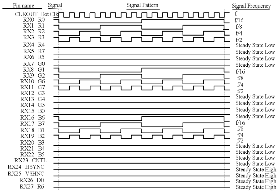
FIGURE 3. TTL Output
