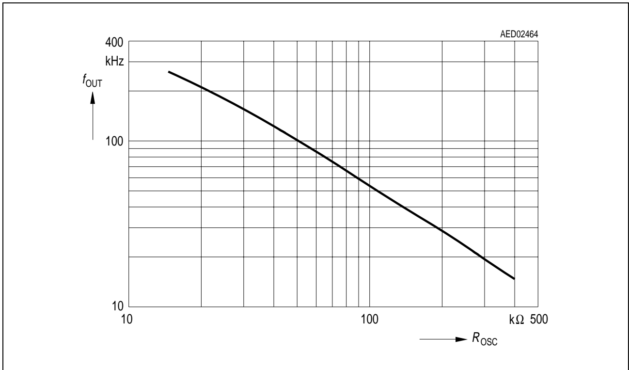
Figure 5 PFC/PWM Frequency
