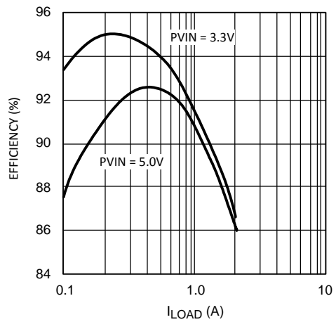
Figure 3. Efficiency vs I_{Load} V_{OUT} = 2.5\text{ V}
