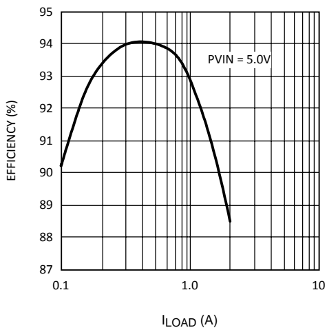
Figure 4. Efficiency vs I_{Load} V_{OUT} = 3.3\text{ V}
