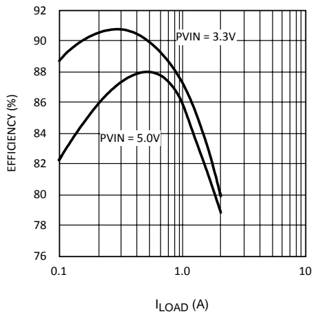
Figure 2. Efficiency vs I_{Load} V_{OUT} = 1.5\text{ V}
