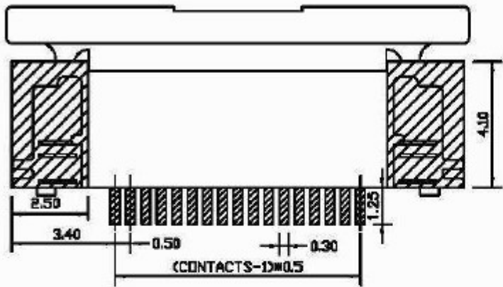
ZIF Connector 32 pins, 0.5mm pitch, Top contact
