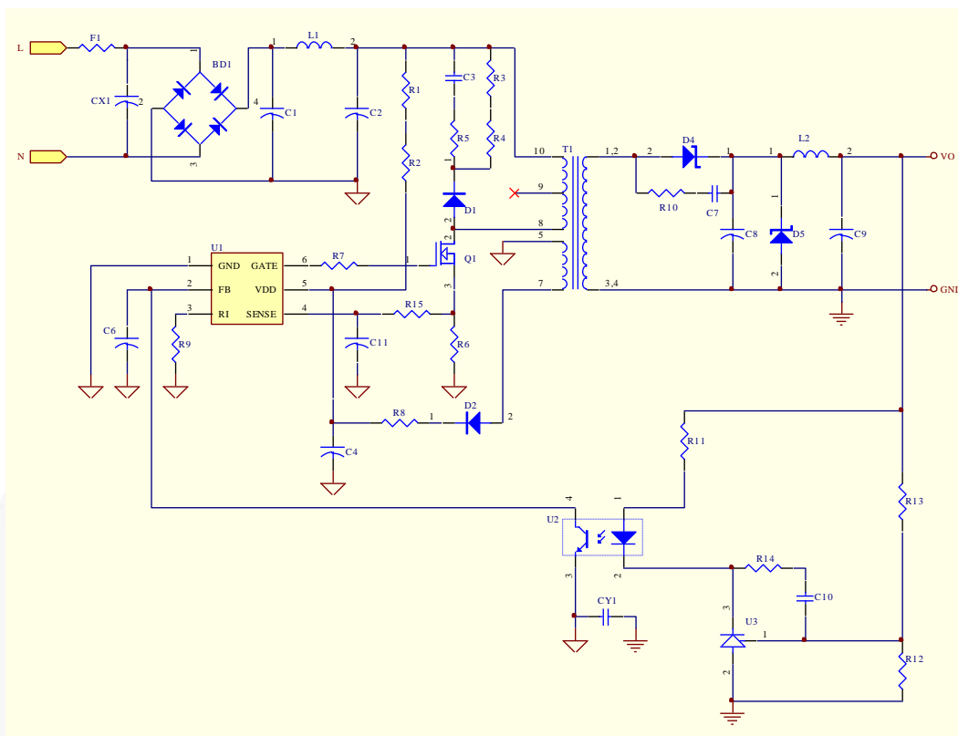
Figure 16. Reference Circuit
