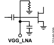
Figure 9. VGG_LNA Interface Schematic
