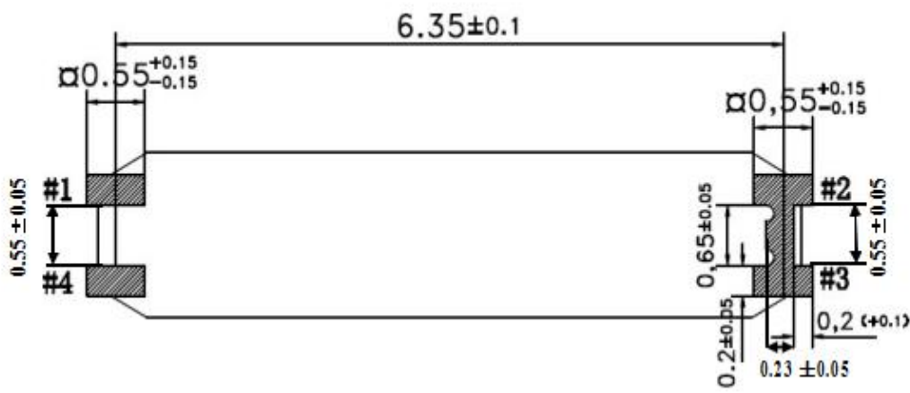
Recommended soldering pattern
