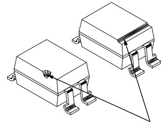
Pin 1 identification
