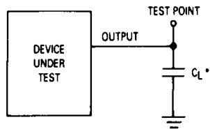
Figure 7. Test Circuit
