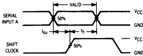
Figure 5. Switching Waveforms
