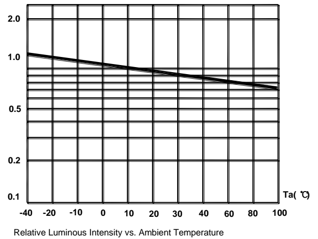
Relative Luminous Intensity vs. Ambient Temperature
