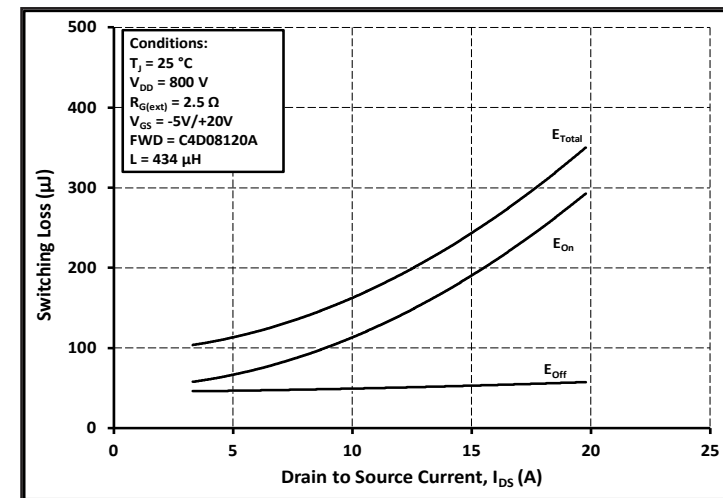
Figure 24. Clamped Inductive Switching Energy vs. Drain Current ( V_{DS} = 600\text{ V} )
