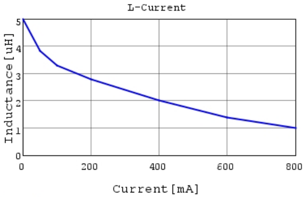
LQM21PN4R7NGR L-Current 20degC
