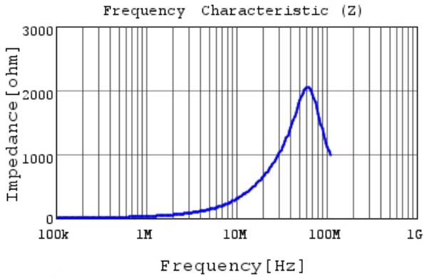
LQM21PN4R7NGR |Z|
