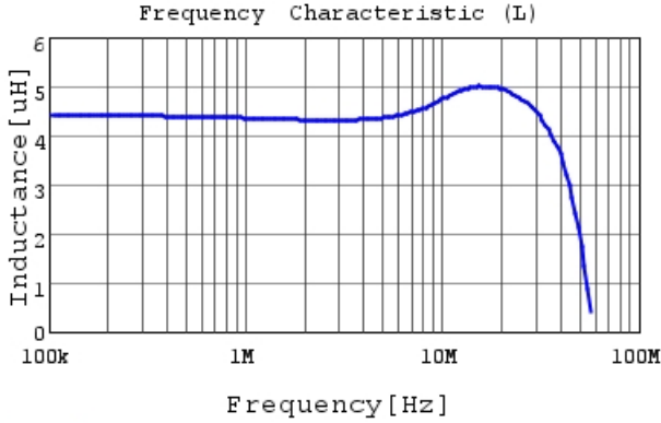
LQM21PN4R7NGR L
