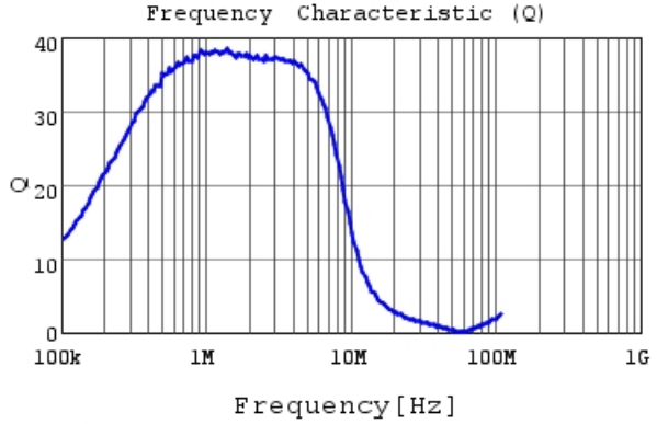
LQM21PN4R7NGR Q
