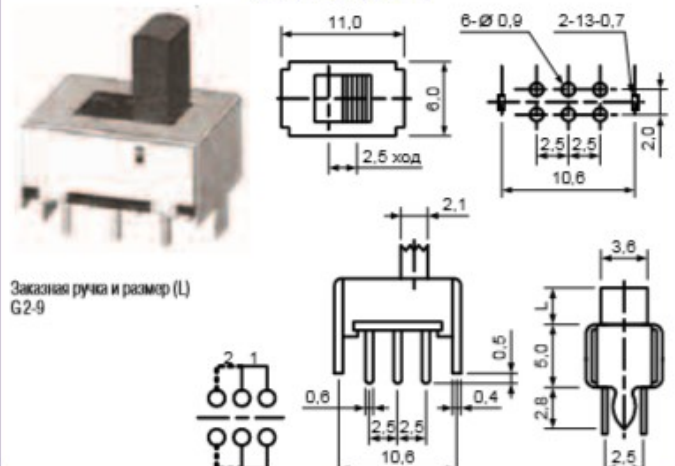
SS22F48(2P2T)
