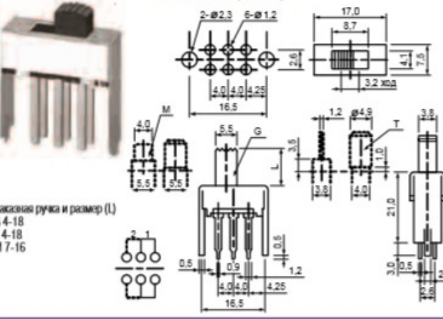
SS22F51(2P2T)
