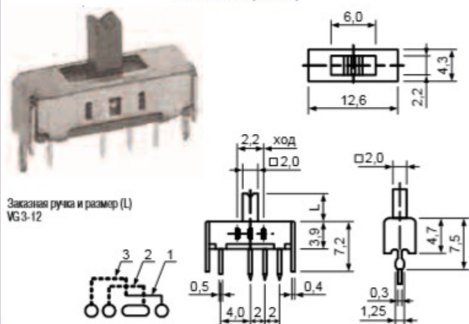
SS22E01(2P2T)
