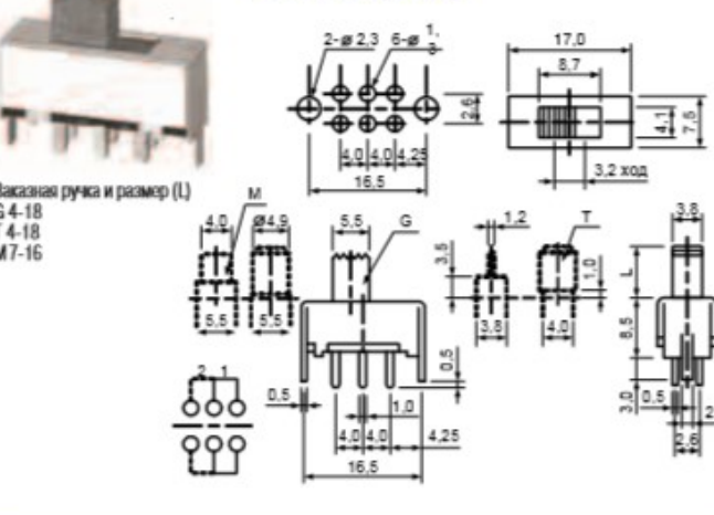
SS22F51(2P2T)
