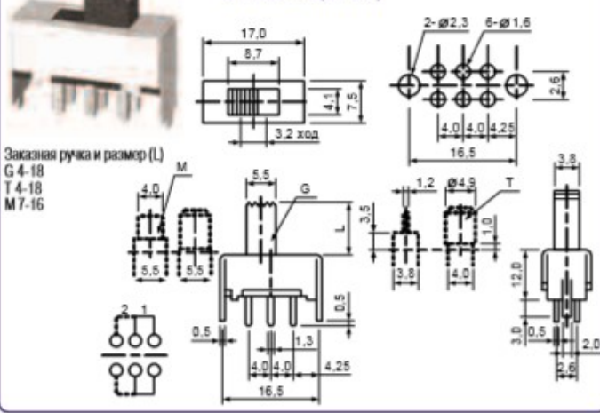
SS22F48(2P2T)
