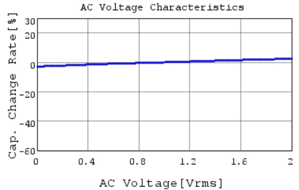
RDER71H104K0K1H03B C-AC Voltage capchange, I
