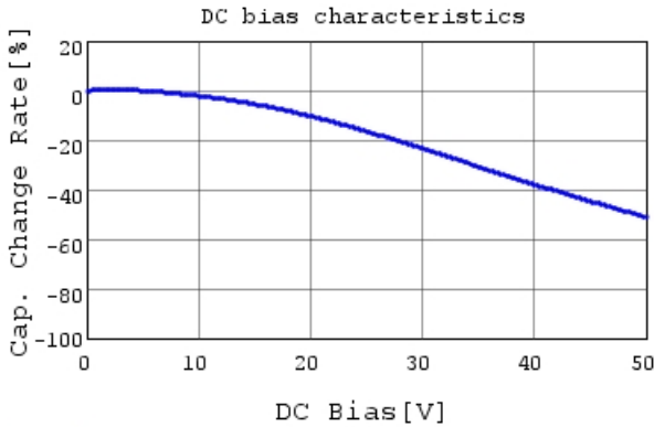
RDER71H104K0K1H03B C-DC bias capchange, 25.0
