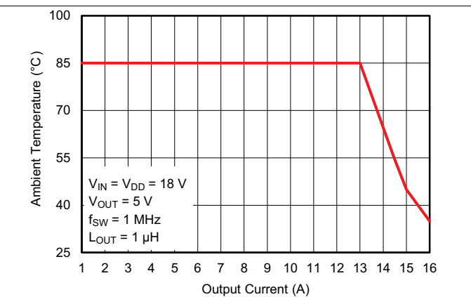
Figure 12. Safe Operating Area, V_{OUT} = 5 \text{ V}
