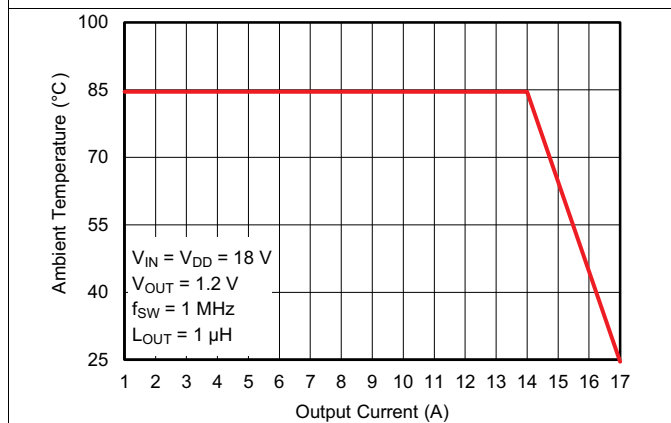
Figure 11. Safe Operating Area, V_{OUT} = 1.2 \text{ V}
