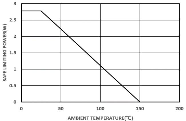
Figure 6. Thermal Derating Curve, Dependence of Safety Limiting Values with Ambient Temperature per VDE (left: \pi 14xM3x ; right: \pi 14xM6x )
