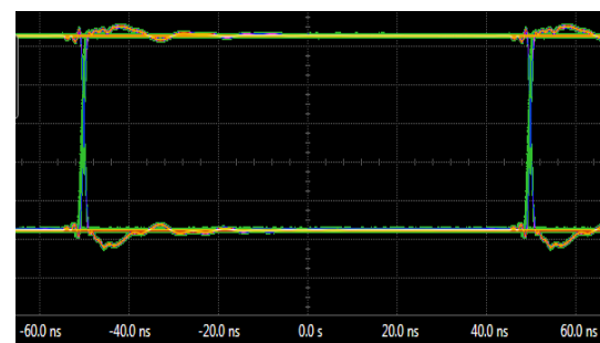
Figure 13. \pi 14xMxx Eye Diagram
