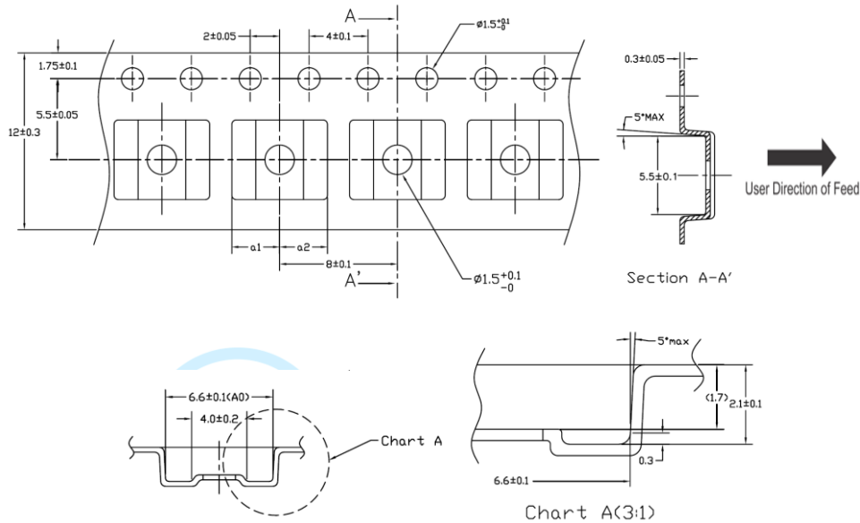
Figure 24. 16-Lead SSOP [SSOP-16] Reel Information—dimension unit(mm)
