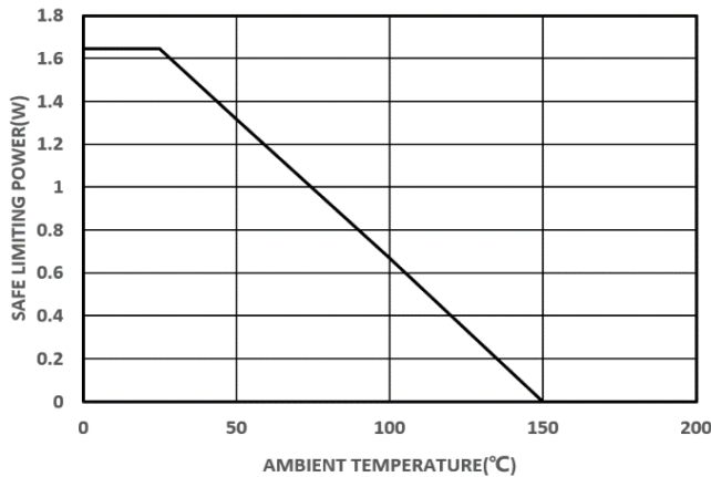
Figure 6. Thermal Derating Curve, Dependence of Safety Limiting Values with Ambient Temperature per VDE (left: \pi 14xM3x ; right: \pi 14xM6x )
