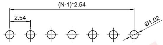
Recommend PCB Layout (Tolerance:±0.05)
