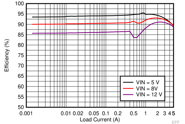
Figure 9-10. LM73605-Q1 Efficiency
