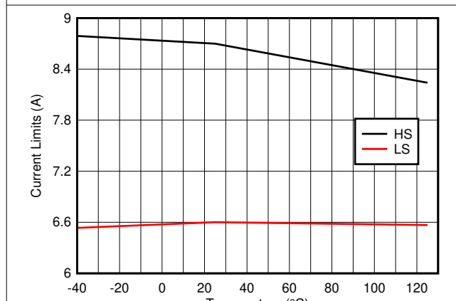
Figure 7-5. LM73605-Q1 High-Side and Low-Side Current Limit
