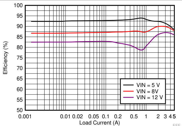
Figure 9-5. LM73605-Q1 Efficiency
