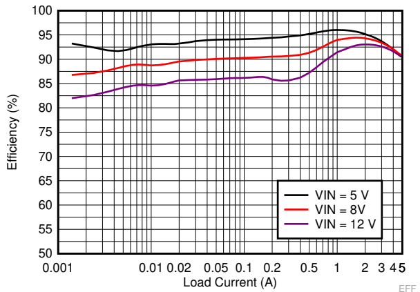
Figure 9-3. LM73606-Q1 Efficiency
