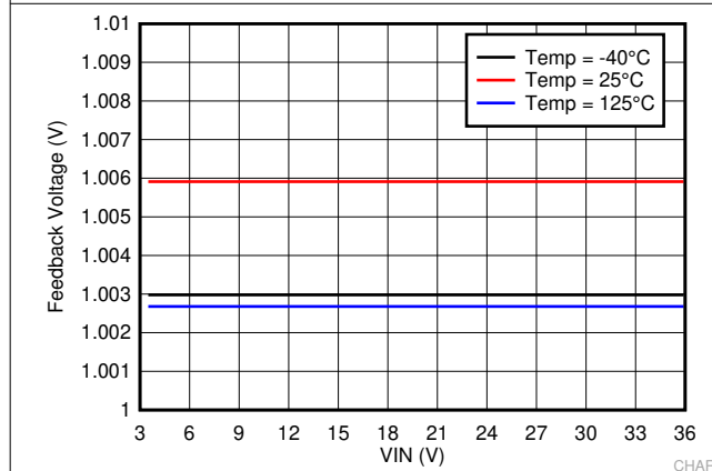
Figure 7-3. Feedback Voltage
