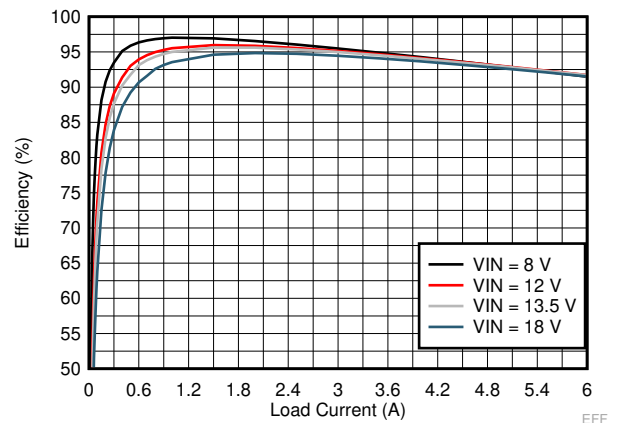
Figure 9-10. LM73605-Q1 Efficiency
