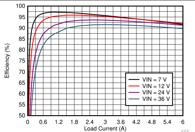
Figure 9-12. LM73606-Q1 Efficiency
