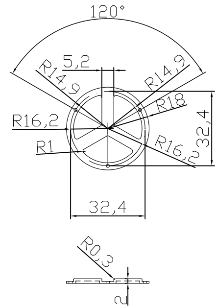
Rubber Button
