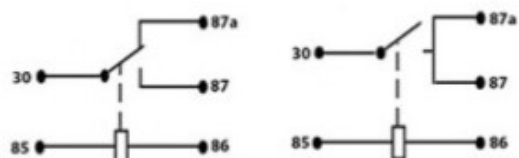
FORM C
