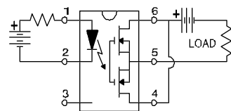
"C" Connection
