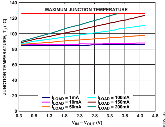
Figure 57. WLCSP, T_A = 85^\circ\text{C}
