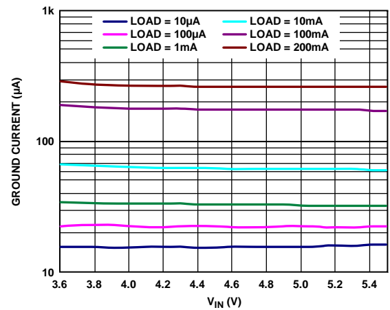
Figure 12. Ground Current vs. V_{IN}
