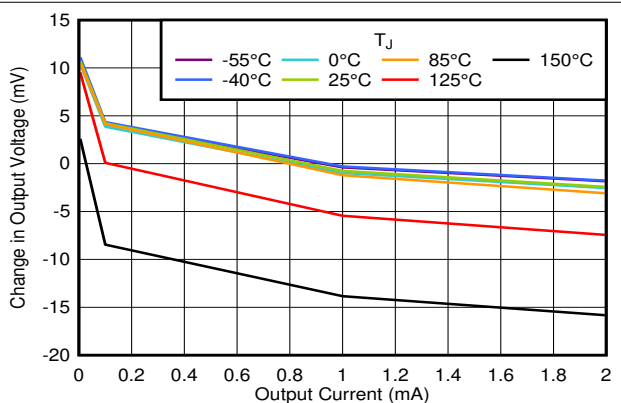
V_{OUT} = 5.5 \text{ V} , V_{EN} = 1 \text{ V} , DQN, YCJ, and YCK packages Figure 6-10. Load Regulation vs I_{OUT}
