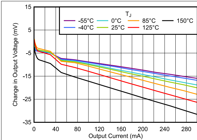
V_{IN} = 2.8 \text{ V} , V_{EN} = 1 \text{ V} , DBV package Figure 6-7. Load Regulation vs I_{OUT}
