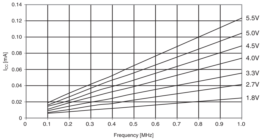
Figure 29-486. Reset Supply Current vs. Low Frequency
