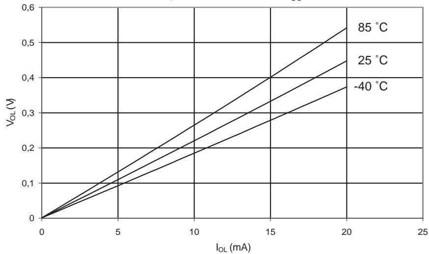
Figure 29-416. I/O Pin Output Voltage vs. Sink Current ( V_{CC} = 5V ).
