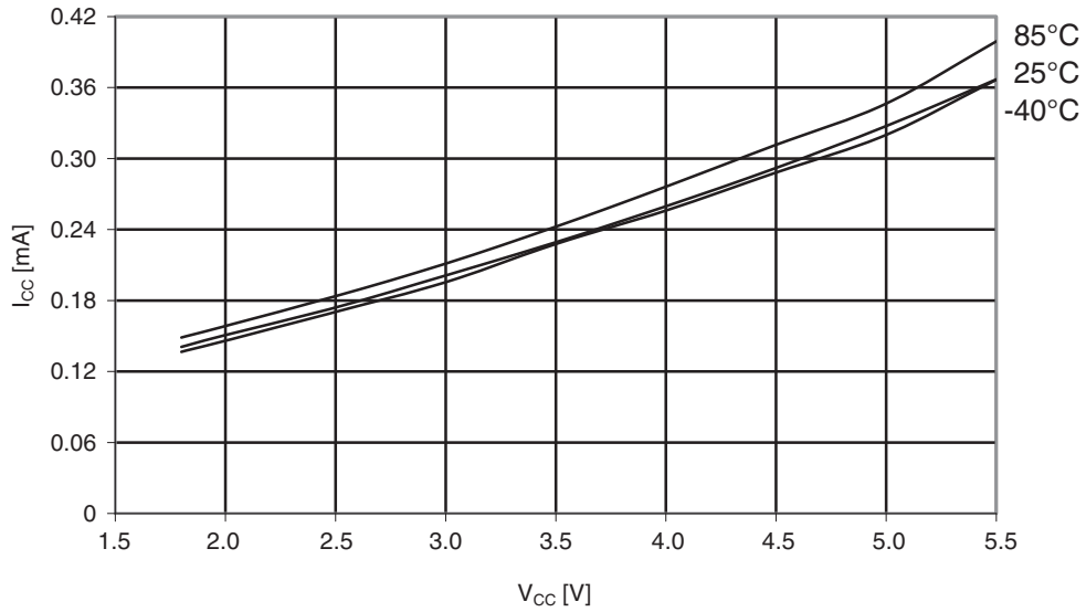
Figure 29-353. Atmel ATmega1284P: Idle supply current vs. V_{CC} (internal RC oscillator, 1MHz).
