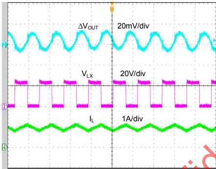
Time (2μs/div)
