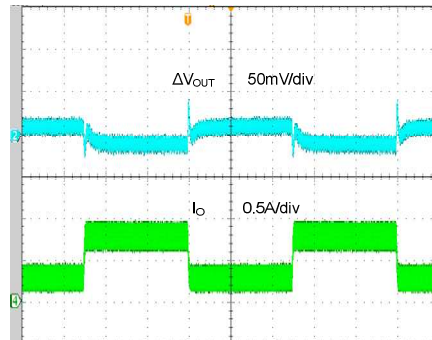
Time (400μs/div)
