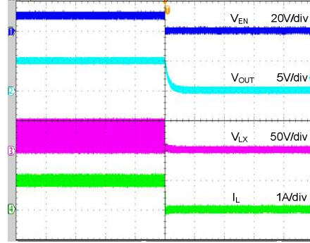
Time (400µs/div)
