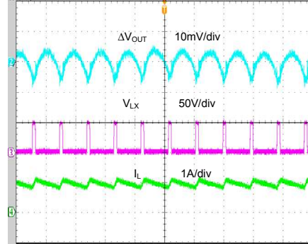
Time (2μs/div)
