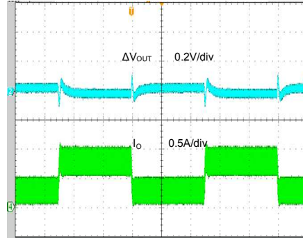
Time (400μs/div)
