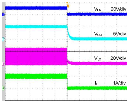
Time (400µs/div)
