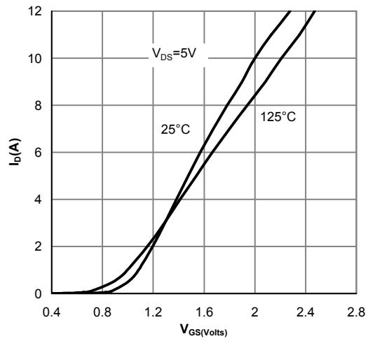
Figure 2: Transfer Characteristics
