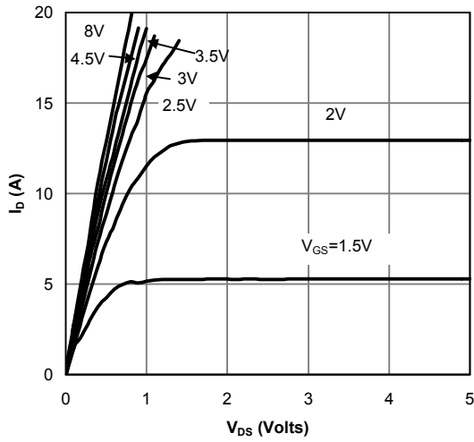
Fig 1: On-Region Characteristics
