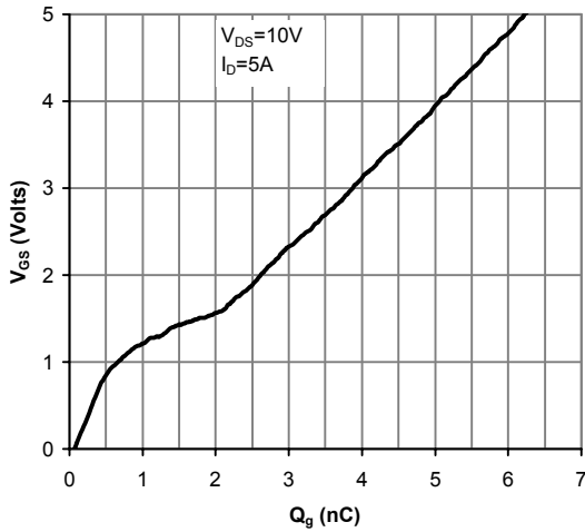
Figure 7: Gate-Charge Characteristics
