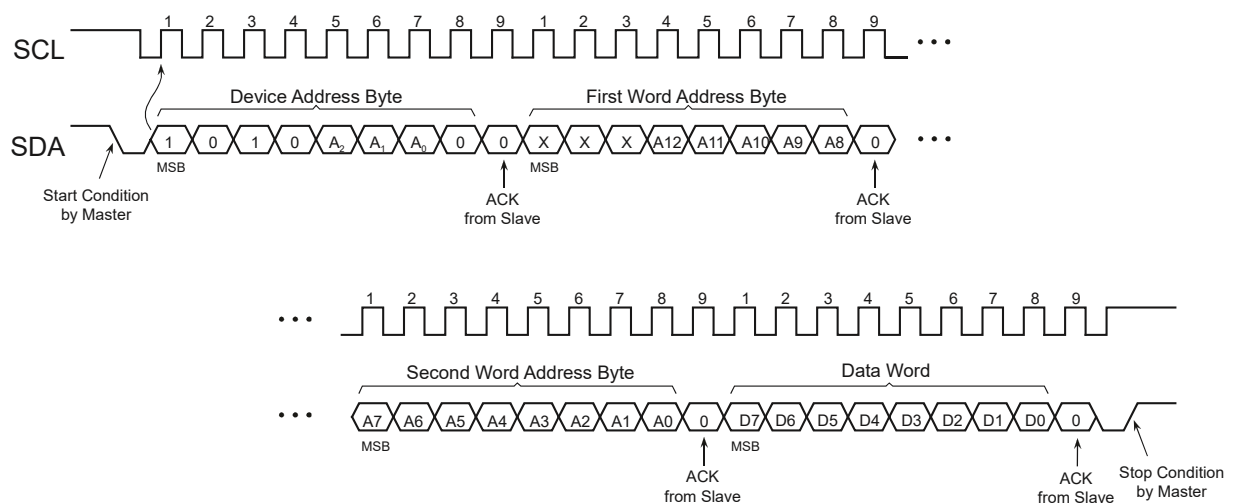
Figure 5-1. Byte Write
