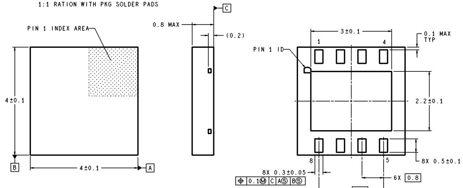
8-Lead LLP Order Part Number LM3940LD-3.3 NSC Package Number LDC08A
