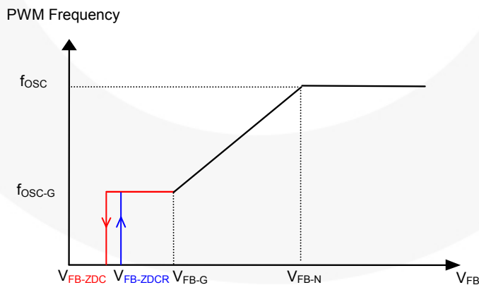
Figure 5. V_{FB} vs. PWM Frequency
